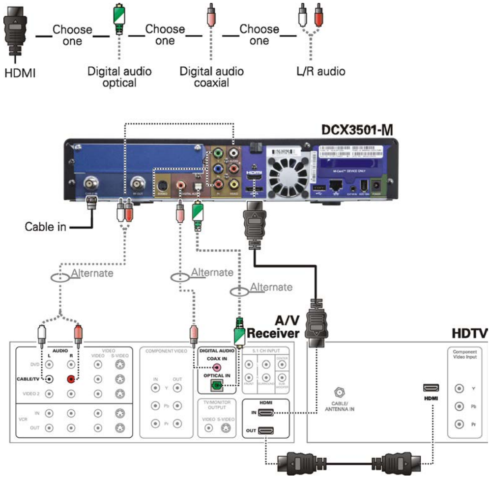
Figure 6 – Connecting the DCX to an A/V receiver – audio
